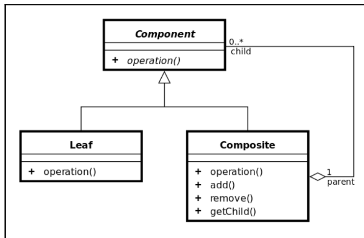
UML diagram for the Composite Design Pattern
