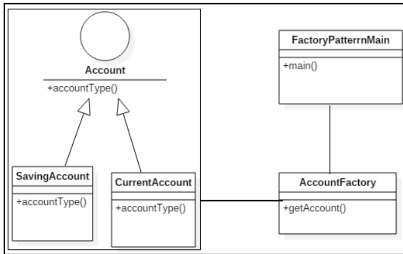
UML Diagram for the Factory design pattern
