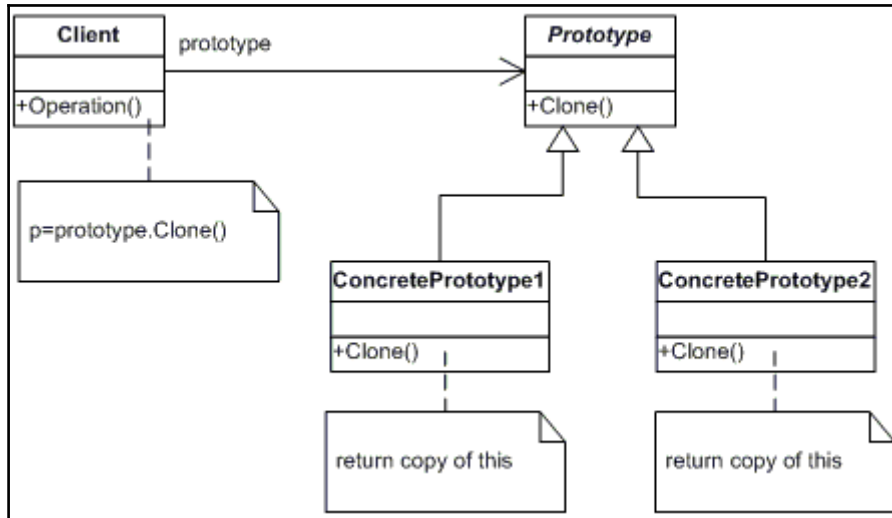
UML diagram for Prototype design pattern
